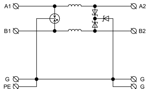
Internal diagram
